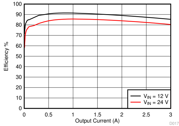
Figure 2-1. TPS54334EVM-722 Efficiency
