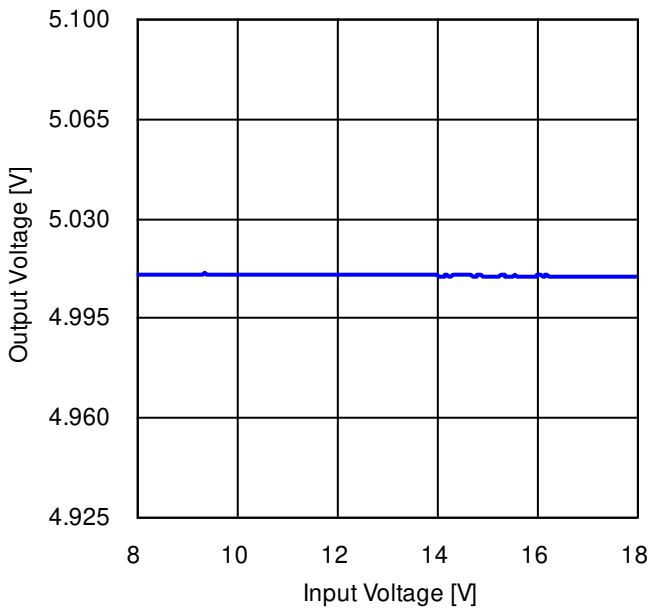
Figure 86. Line Regulation ( I_{OUT} = 2\ \text{A} )
