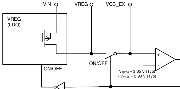
Figure 38. VCC_EX Block Diagram
