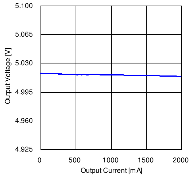
Figure 87. Load Regulation ( V_{IN} = 12\ \text{V} )
