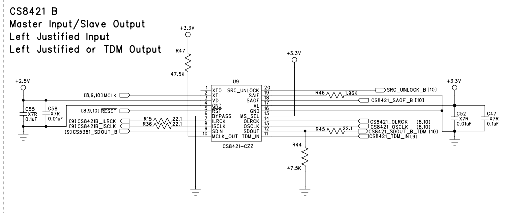
Figure 12. CS5381 & CS8421 Pair B
