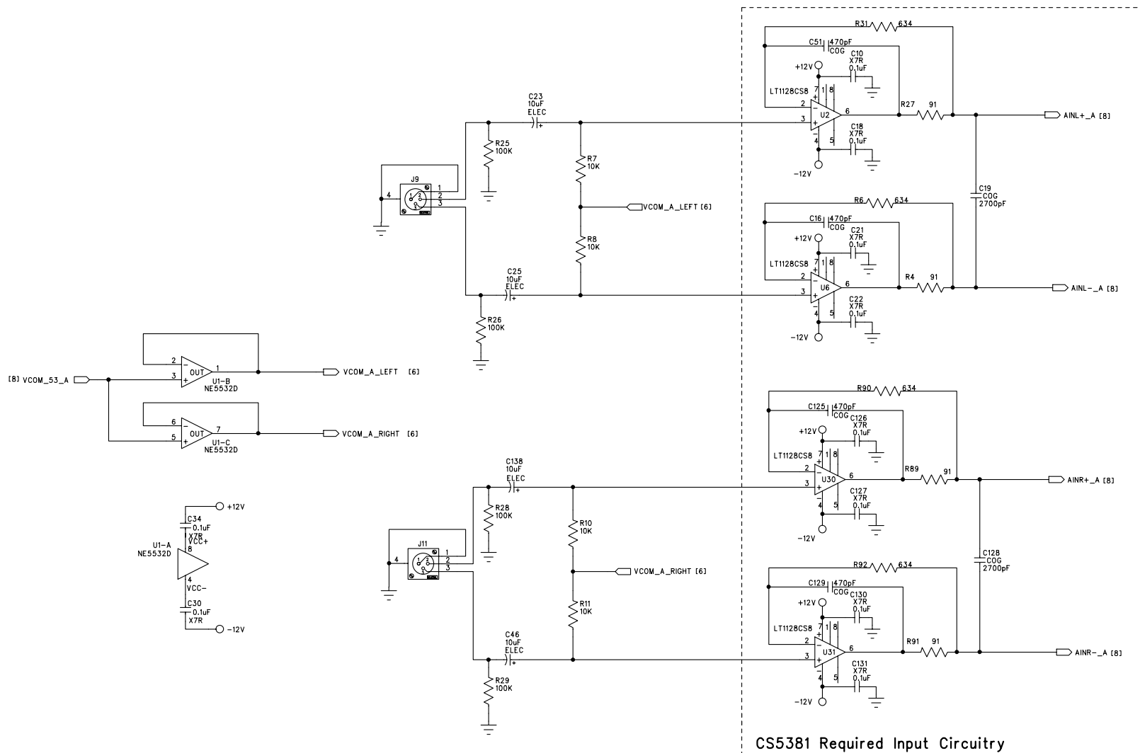
Figure 9. Analog Inputs 1 &amp; 2
