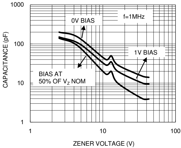
Fig.5 Typical Capacitance
