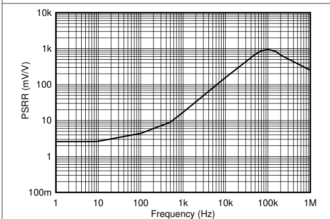
Figure 7-11. PSRR vs. Frequency
