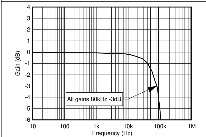
Figure 7-9. Sensitivity vs. Frequency, All Gains Normalized to 1 Hz
