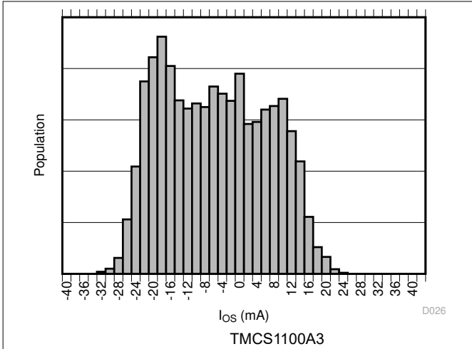
Figure 7-7. Input Offset Current Production Distribution
