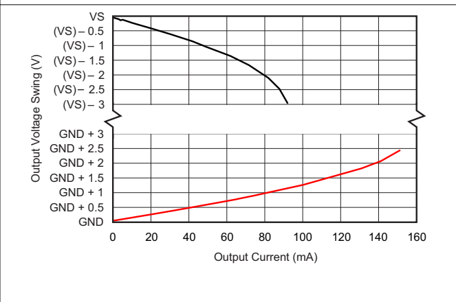
Figure 7-12. Output Swing vs. Output Current
