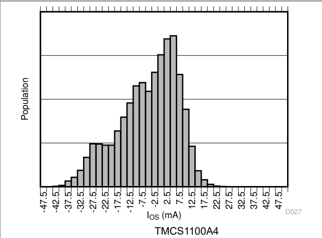
Figure 7-8. Input Offset Current Production Distribution
