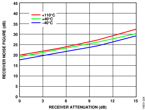
Figure 183. Receiver Noise Figure vs. Receiver Attenuation, 5600 MHz LO, 100 MHz Bandwidth, 122.88 MSPS Sample Rate, 50 MHz Integration Bandwidth (Includes 1.2 dB Matching Circuit Loss)
