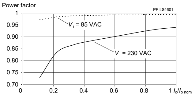
Fig. 7 Power factor versus output current (LS4601-7R)
