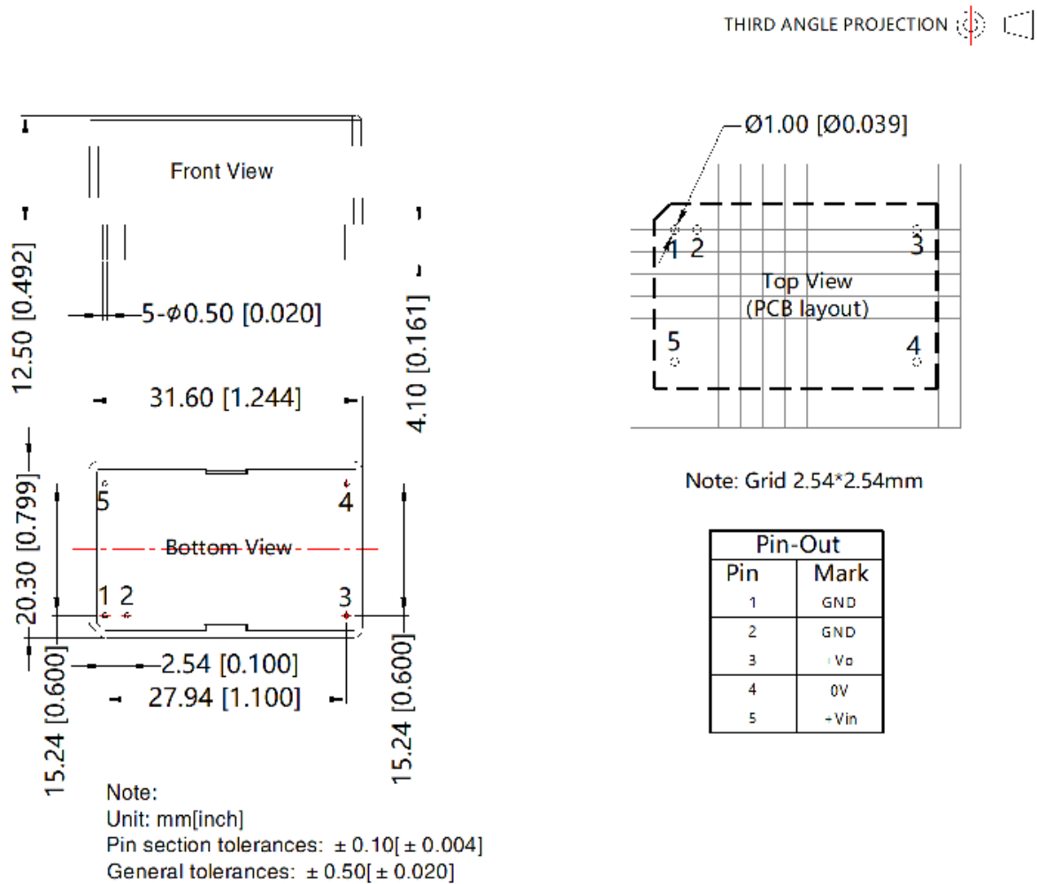
Figure 5. Mechanical Drawing of Standard Model
