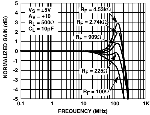
FIGURE 13. GAIN vs FREQUENCY FOR VARIOUS R_F ( A_V = +10 )
