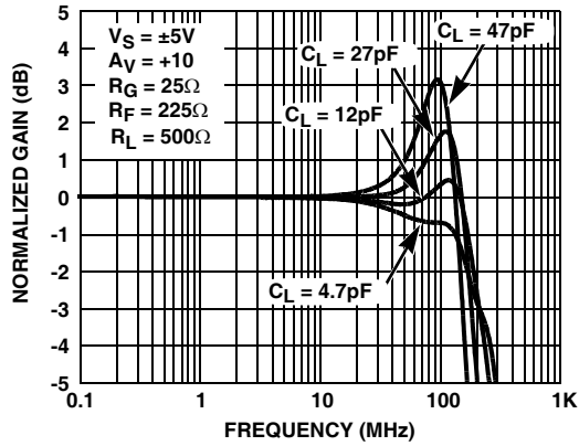
FIGURE 11. GAIN vs FREQUENCY FOR VARIOUS C_{LOAD} ( A_V = +10 )
