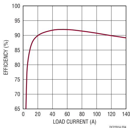
Figure 4. Typical Efficiency Curves of DC2291A, V_{IN} = 12V , V_O = 1.0V , F_{SW} = 450kHz , CCM
