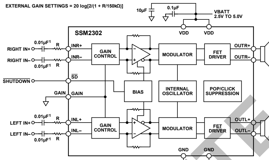
Figure 24. Stereo Differential Input Configuration, User-Adjustable Gain
