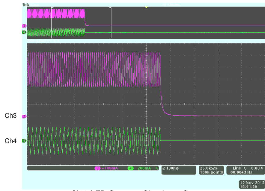
Figure 7. Enable Turn Off Waveform
