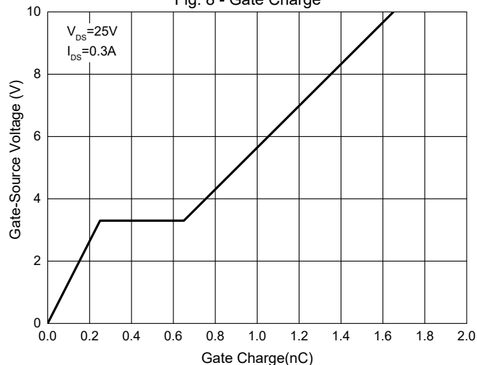
Fig. 8 - Gate Charge
