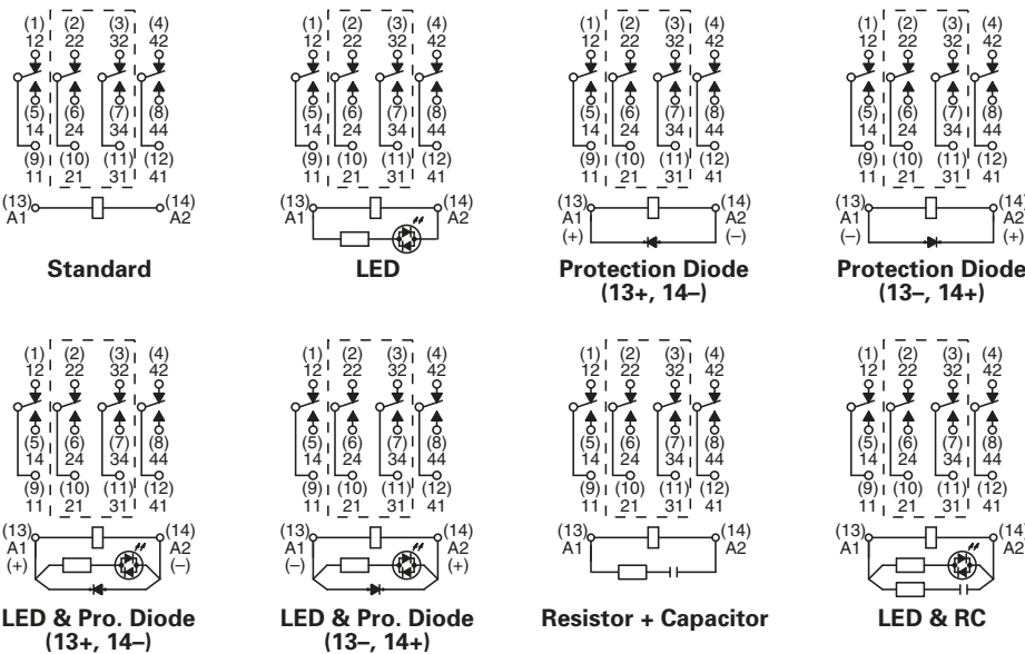
4 Pole Models
