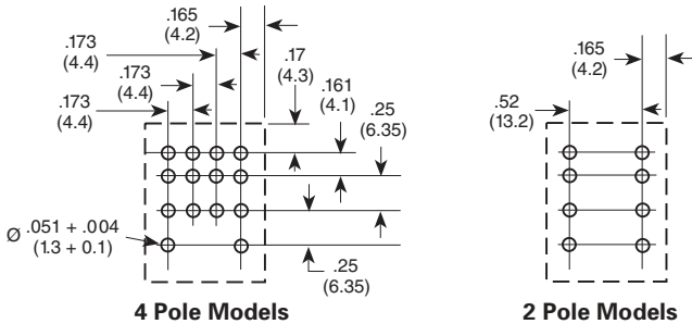
4 Pole Models
