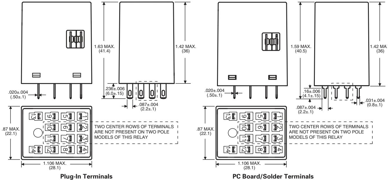
Plug-In Terminals
