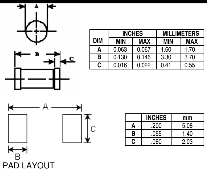
PAD LAYOUT
