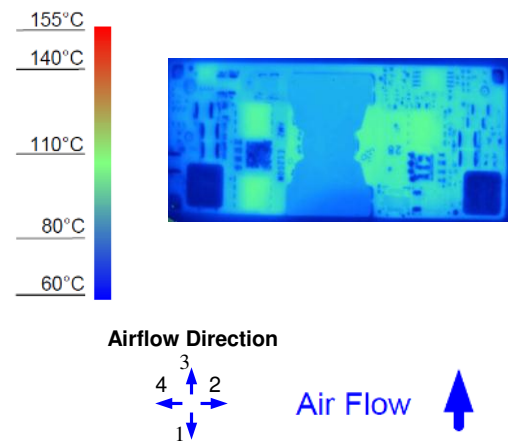
Figure 8. Thermal Image for Airflow Direction 3 (4A output, 55°C ambient, 200 LFM, typical Vin, open frame)
