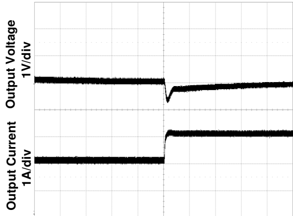
Time - t (500µs/div)
