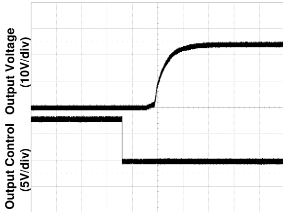
Time - t (5ms/div)
