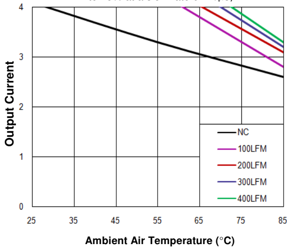
Figure 7. Current Derating Curve for Airflow Direction 3 (Ref. Figure 8 for Airflow Direction; Vin = 36V, open frame unit)
