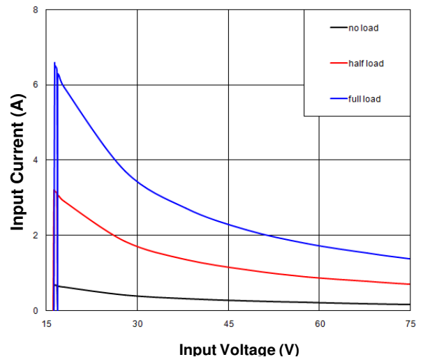
Figure 2. Input Characteristics
