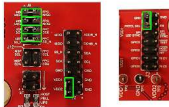
Figure 4. SPI Configuration
