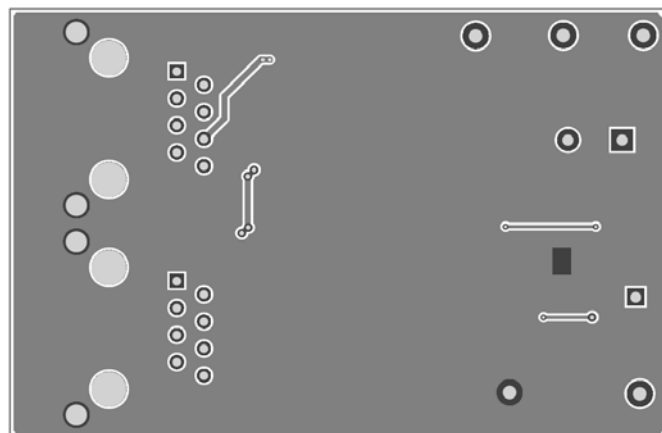
Figure 3: Bottom Layer
