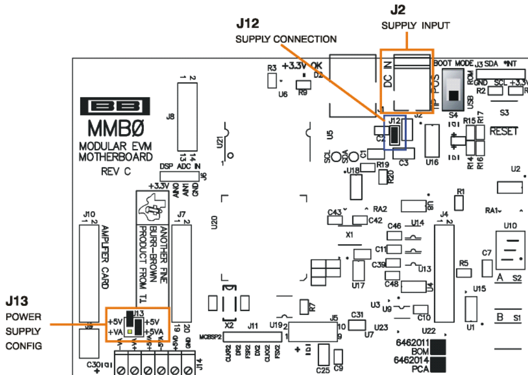
Figure 4. Connecting an External Power Supply
