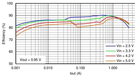
Figure 9-2. Efficiency
