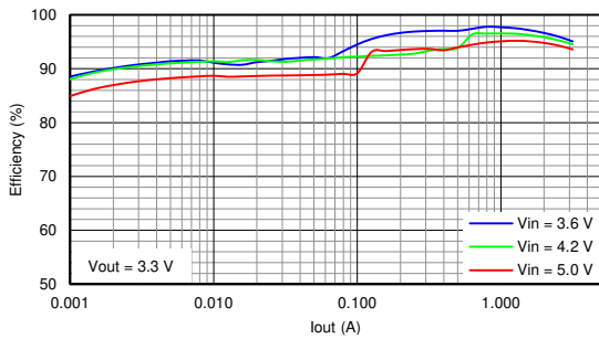
Figure 9-4. Efficiency
