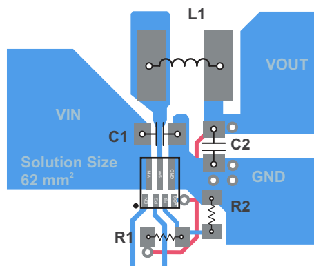
Figure 11-1. PCB Layout Recommendation
