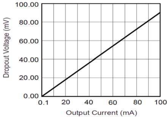
Figure 17. Dropout Voltage
