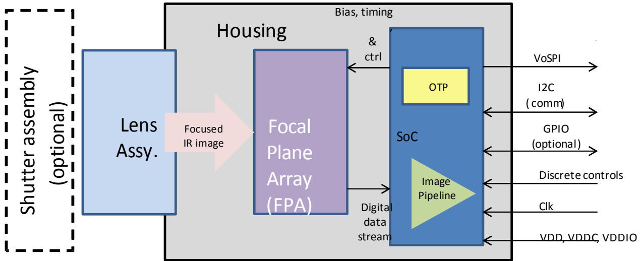
Figure 4 - Lepton 3 Architecture
