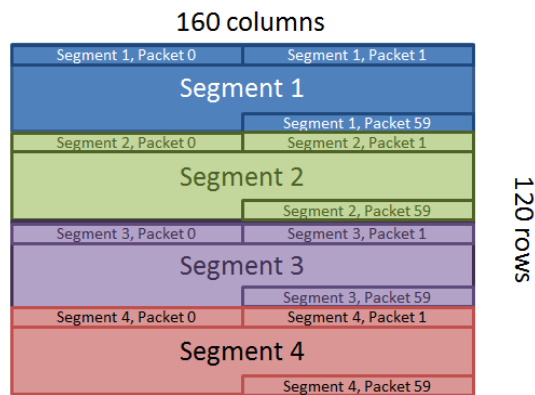
(a) Frame contents with telemetry disabled
