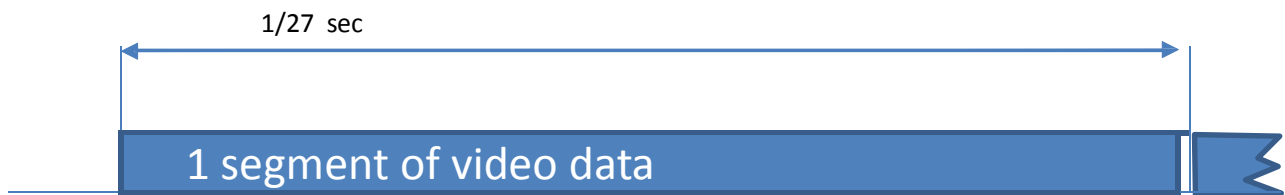
Figure 17 - VoSPI Flexible Clock Rate
