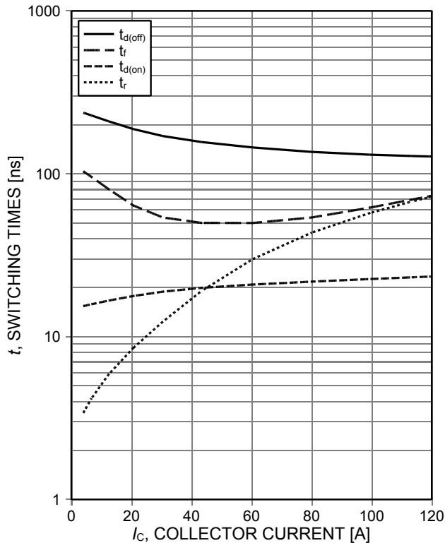
Figure 7. Typical switching times as a function of collector current (ind. load, T j =150°C, V CE =400V, V GE =0/15V, R G =10Ω, test circuit in Fig. E)
