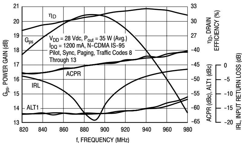
Figure 3. Single-Carrier N-CDMA Broadband Performance @ P out = 35 Watts Avg.
