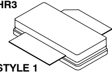
CASE 465A-06, STYLE 1 NI-780S MRFE6S9160HSR3
