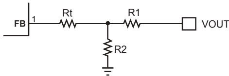
Figure 3— T-type Network
