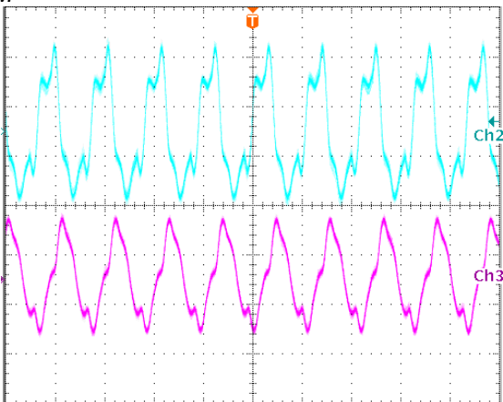
Output voltage ripple at nominal input voltage and max load current Top trace +15V, 10mV/div, Bottom trace -15V, 20mV/div, 2us/div. Load cap: 10 \mu F, tantalum capacitor and 1 \mu F ceramic capacitor. Bandwidth: 20MHz.
