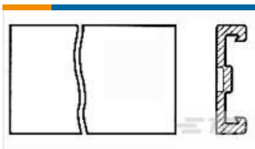
TE Part #640643-7 07P MTA156 COVER F/T
