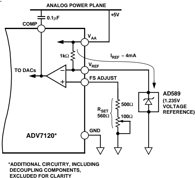
Figure 4. Reference Circuit
