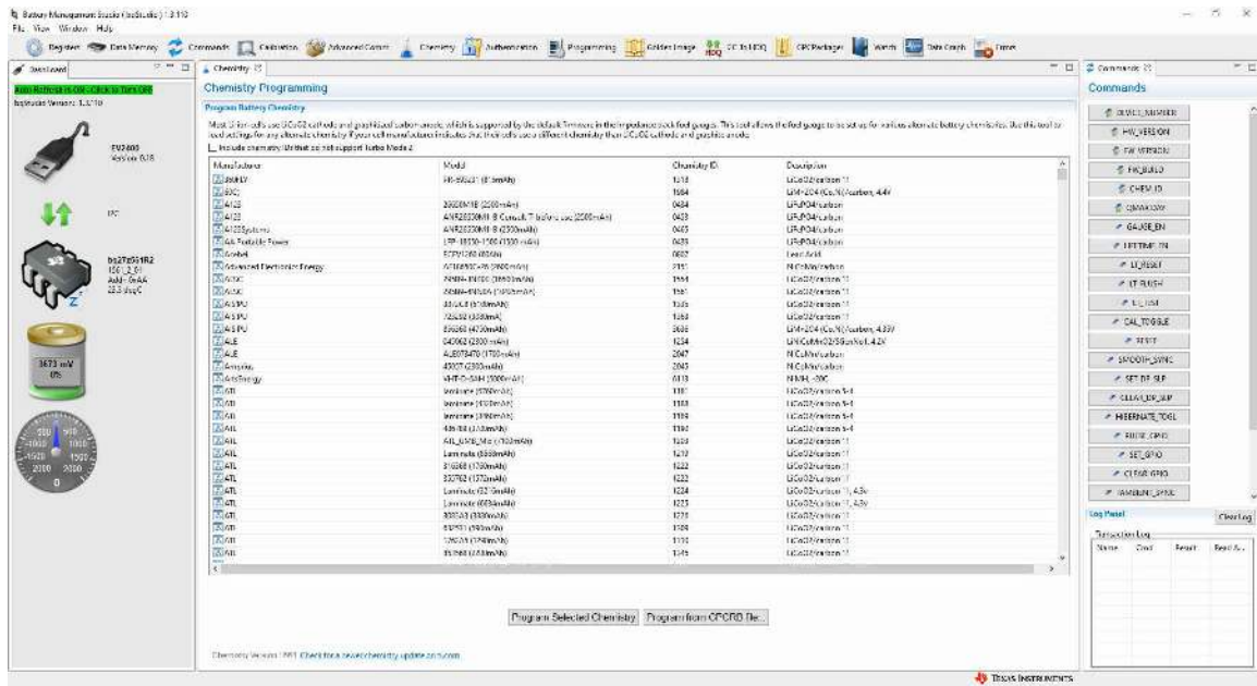
Figure 7-3. Chemistry Screen
