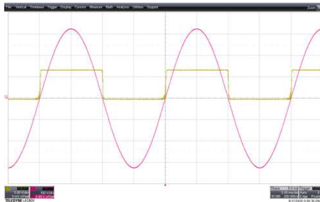
Figure 11 – 230 VAC 50 Hz. CH1: ZCD, 5 V / div., 5 ms / div. CH2: V_{IN} , 100 V / div., 5 ms / div.
