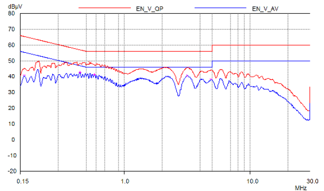
Figure 51 – 230 VAC 60 Hz.
