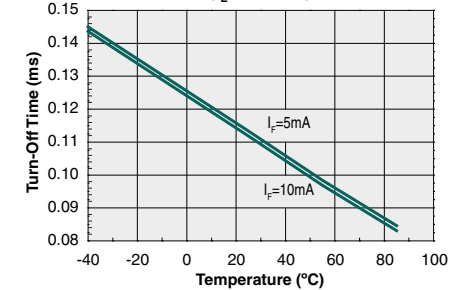
Turn-Off Time vs. Temperature ( I_L=100\text{mA} )
