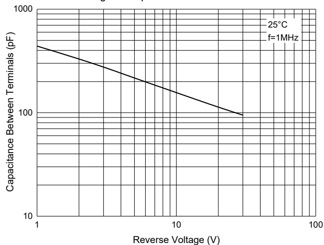
Fig. 2 - Capacitance Characteristics
