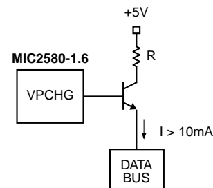
Figure 5. Voltage Source
