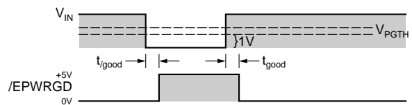
Figure 4. Early Power Good Response Time
