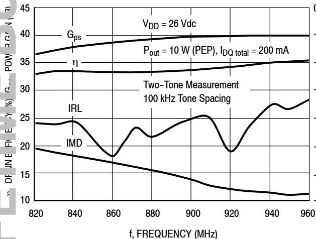
Figure 19. Two-Tone Broadband Performance
