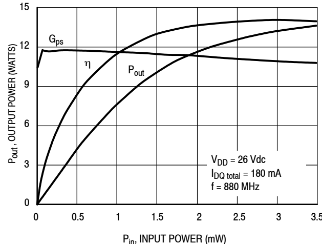
Figure 20. CW Performance @ 880 MHz
