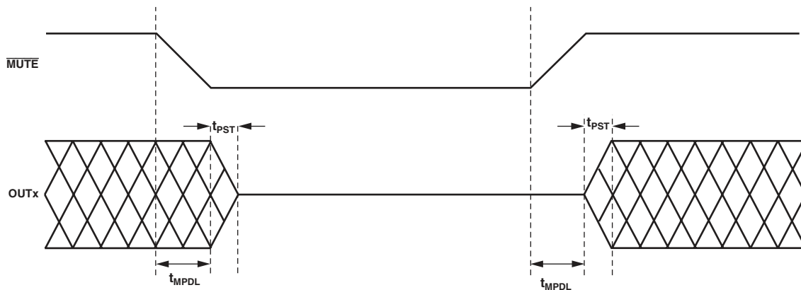
Figure 3. \overline{MUTE} Timing
