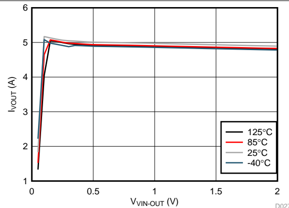
Figure 10. I_{OUT} vs V_{IN-OUT}
