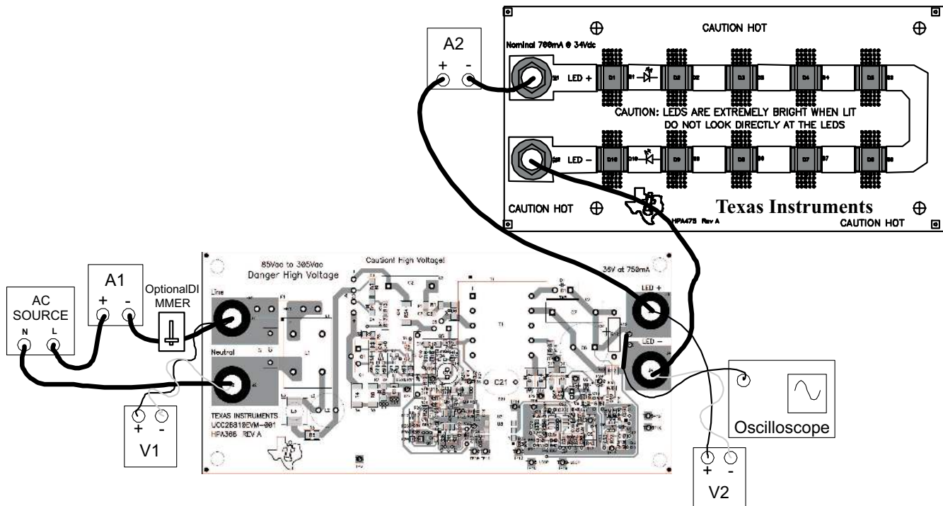
Figure 2. UCC28810EVM-001/HPA475 Recommended Test Set Up
