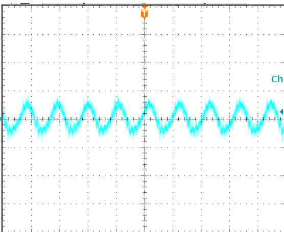
Output voltage ripple at nominal input voltage and max load current (4mV/div, 2us/div) Load cap: 10µF, tantalum capacitor and 1µF ceramic capacitor. Bandwidth: 20 MHz.
