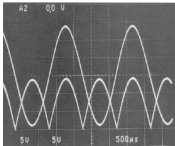
Figure 72. Full Wave Rectifier Waveform
