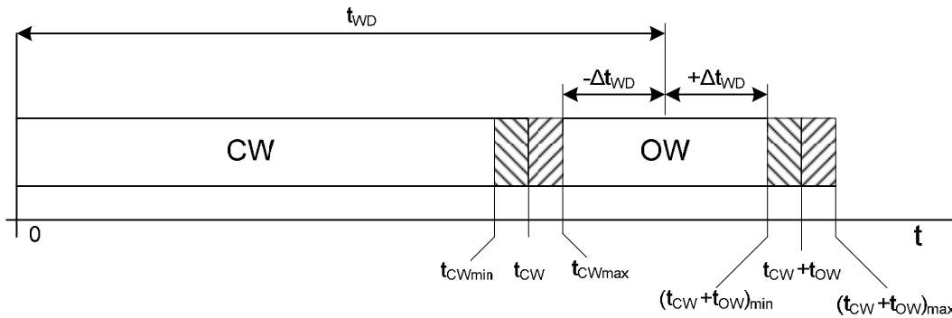
Figure 13: Watchdog open and close window tolerances
