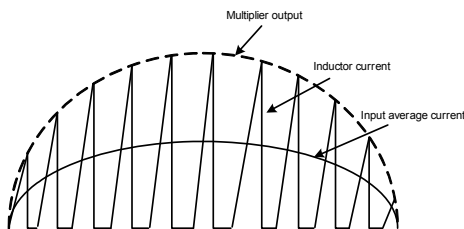
Figure 2: Power-Factor Correction
