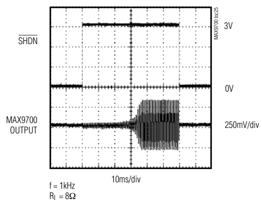
TURN-ON/TURN-OFF RESPONSE
