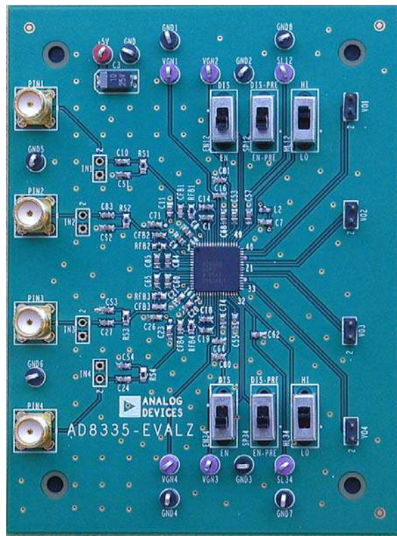
Figure 60. Photograph of the AD8335-EVALZ Evaluation Board
