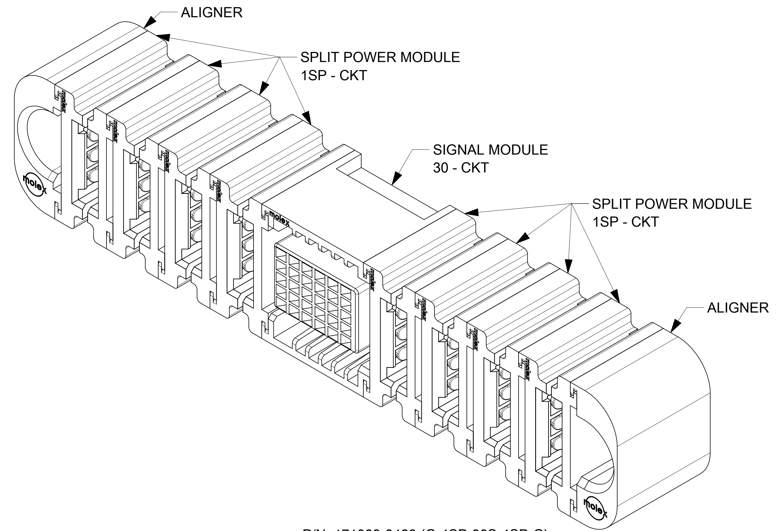
P/N: 171089-8429 (G-4SP-30S-4SP-G)
