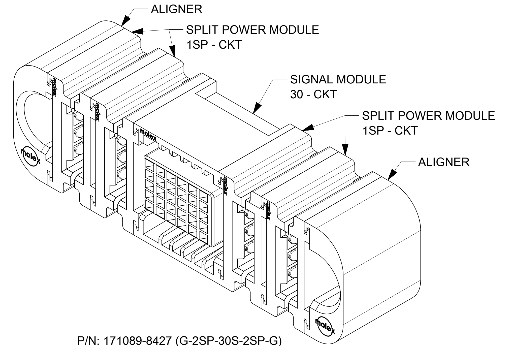
P/N: 171089-8427 (G-2SP-30S-2SP-G)
