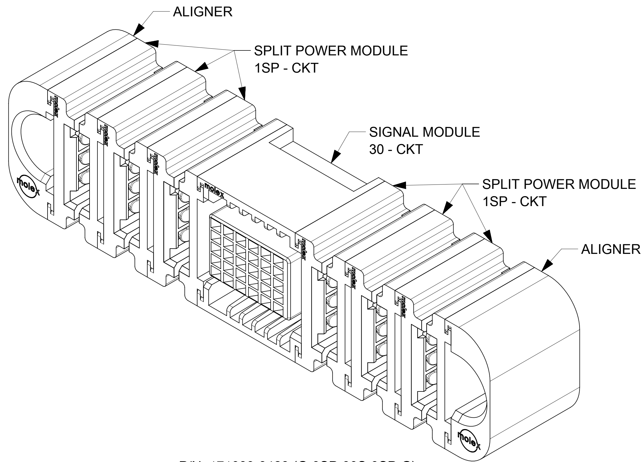
P/N: 171089-8428 (G-3SP-30S-3SP-G)
