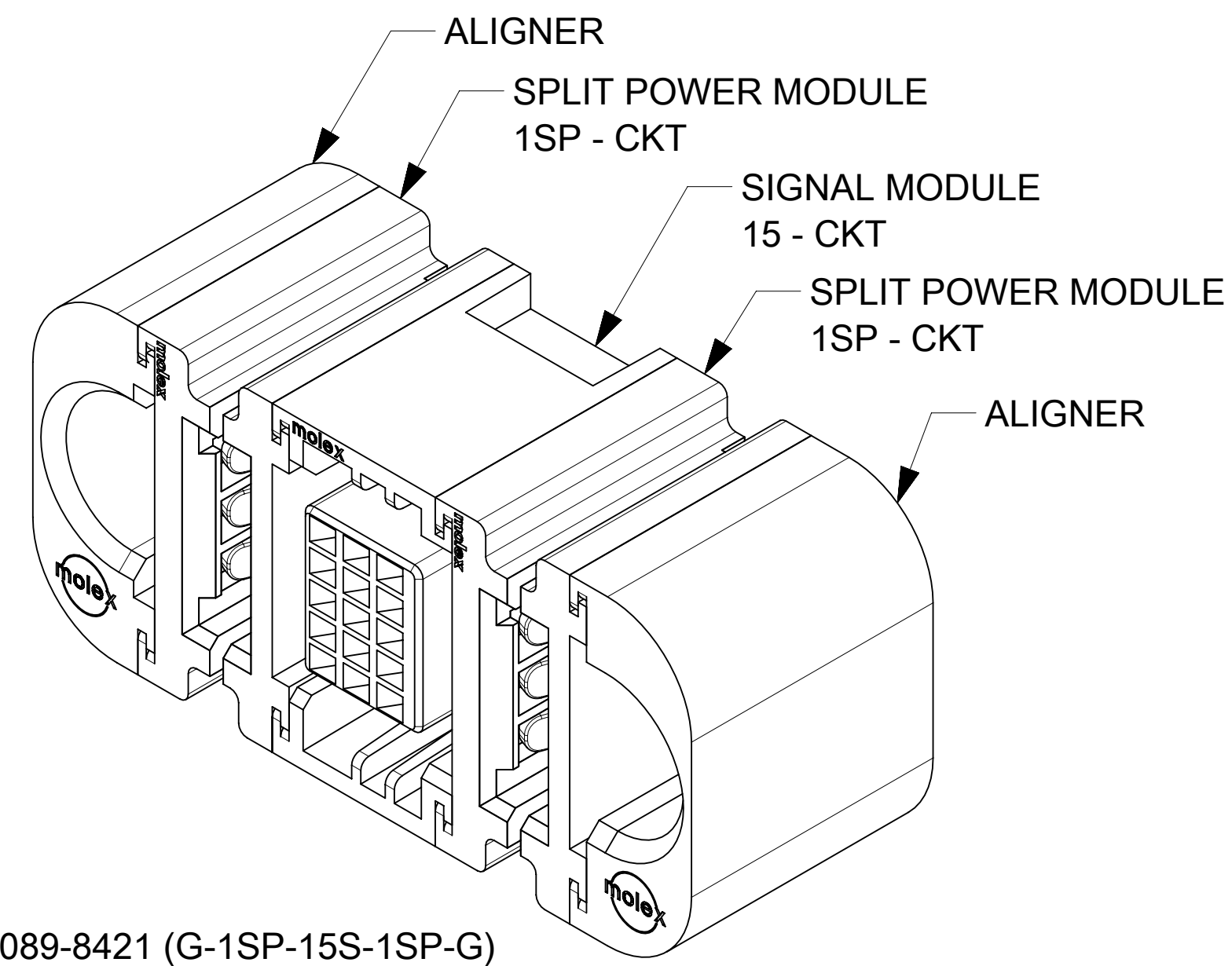
P/N: 171089-8421 (G-1SP-15S-1SP-G)
