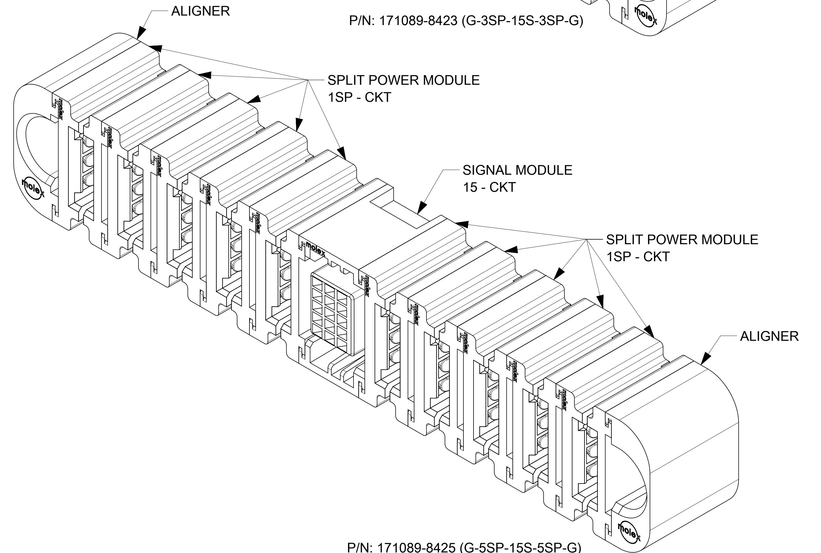
P/N: 171089-8425 (G-5SP-15S-5SP-G)
