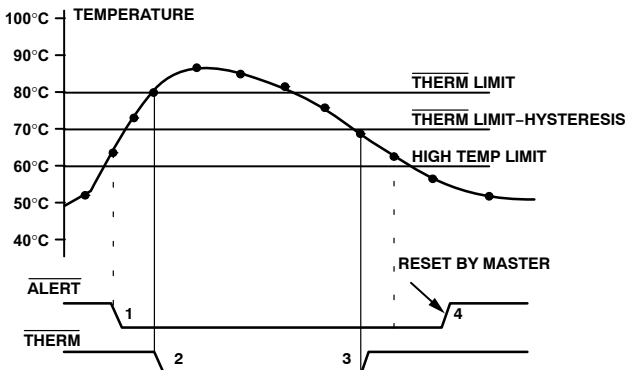
Figure 19. Operation of the \overline{\text{ALERT}} and \overline{\text{THERM}} Interrupts
