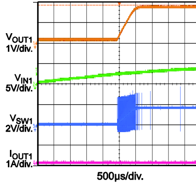
VIN Power On without Load I_{OUT1} = I_{OUT2} = 0A
