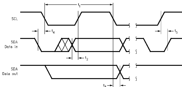
Figure 51. I 2 C Timing Diagram
