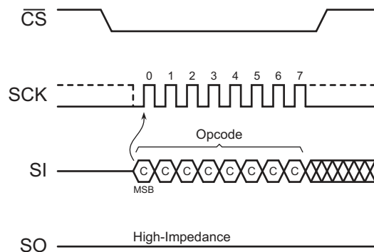
Figure 18. Chip Erase
