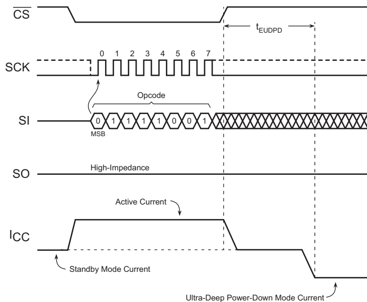
Figure 33. Ultra-Deep Power-Down
