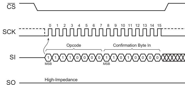
Figure 37. Reset
