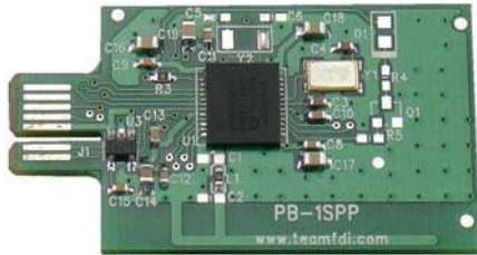
Board Dimensions 1.743" x 0.98"
