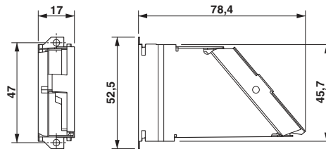
D-SUB EMC inner sleeve
